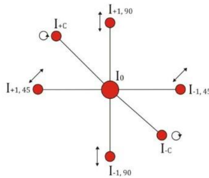
Figure 1. Schematic representation of diffraction orders. I_0 is an 0 order located in the center of an image, the 1st orders of L_{90} grating ( I_{+1,90} and I_{-1,90} ) are positioned in the vertical direction and the 1st orders of L_{45} grating ( I_{+1,45} and I_{-1,45} ) are positioned in the horizontal direction of the image, the 1st orders of C grating ( I_{+C} and I_{-C} ) are positioned with 45^\circ angle to the vertical axes.
