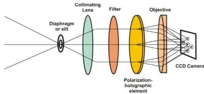
Figure 3. Optical schema of a polarization-holographic Stokes-astropolarimeter.
