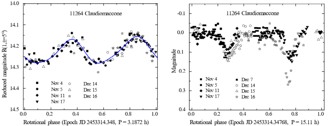
Fig. 6. Observed lightcurves of (11264) Claudiomaccone (Krugly et al., 2007)
