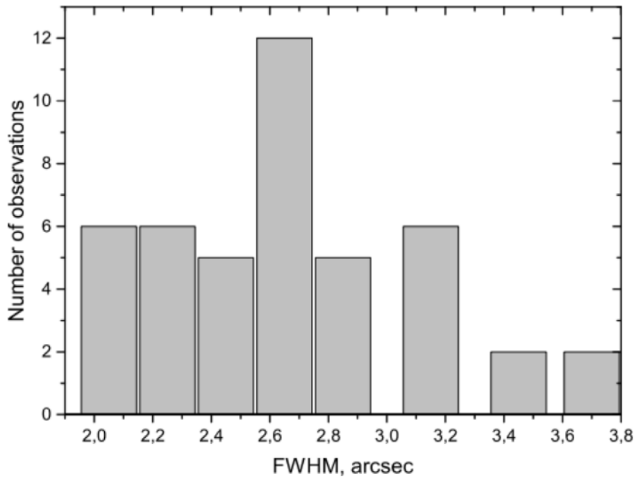
Fig. 1. FWHM distribution of point-like objects in a combined images of GRB afterglow observations presented in Table 1.
