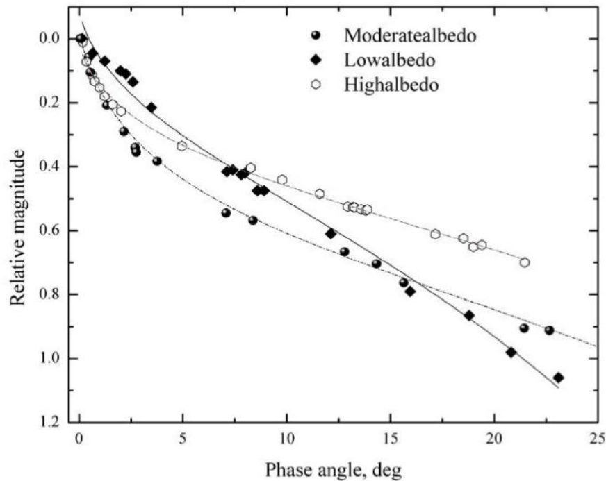
Fig. 8. Relative magnitude-phase relations for high, moderate and low albedo asteroids (Belskaya & Shevchenko 2000)
