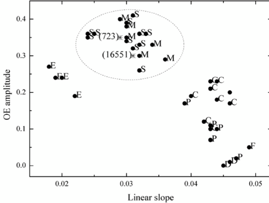
Fig. 9. The relationship of the OE amplitude and the linear slope for asteroids of different types (defined by letters) (Shevchenko et al., 2015)
