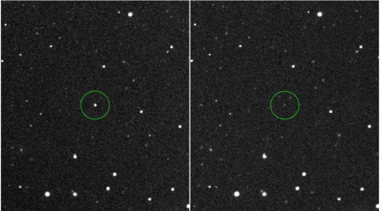
Fig. 2. Observation of the GRB 130427A afterglow with AS-32 telescope on the first day starting 2013-04-27T17:00:57 (left) and on the 3rd days (2013-04-29T16:59:56) after GRB trigger.
