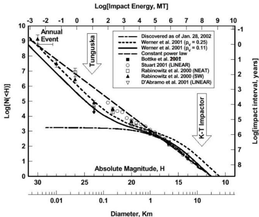
Fig. 1. Cumulative distribution of near-Earth asteroids vs their absolute magnitudes, and a scale for the diameters. Also impact energy and expected impact time interval are shown ( Chapman 2004 ).
