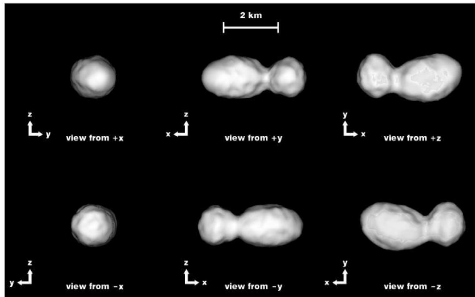
Fig. 5. Reconstructed shape of (8567) 1996 HW1 (Magri et al., 2011).
