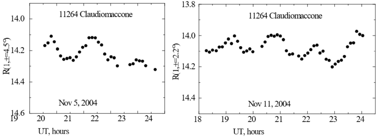
Fig. 6. Observed lightcurves of (11264) Claudiomaccone (Krugly et al., 2007)
